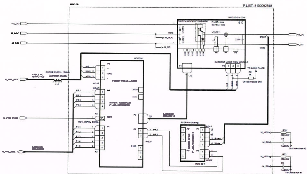
Figure 3 - Main Schematic Pre Charge Switch Converter
